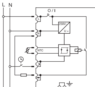
Floor thermostat insert with switch Art. no. 537100
