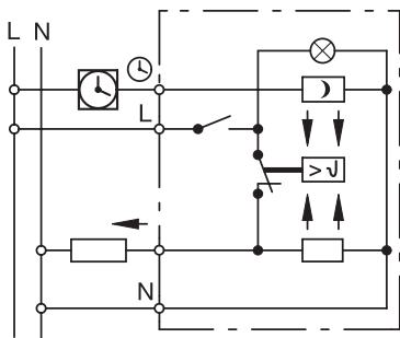
Room temperature control unit insert with switch Art. no. 5363..
