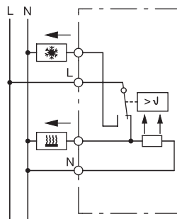
Room temperature control insert with changeover contact Art. no. 5364..
